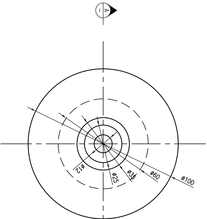
PLAN OF ZGR2 ANODE SCALE 1:1
