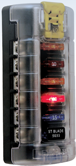
LED ON indicates blown fuse Shown in ST Blade Fuse Block PN 5035
